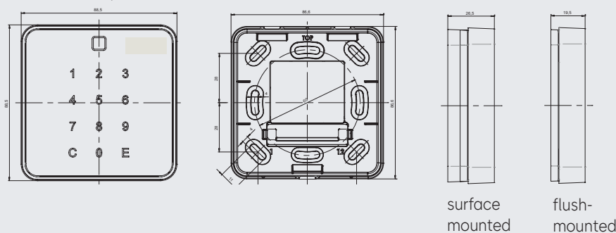
Front and rear panel
