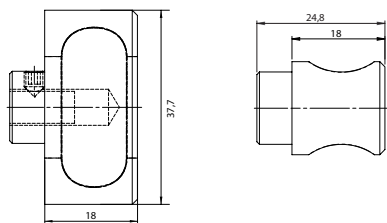
Oval knob (D-Line)
