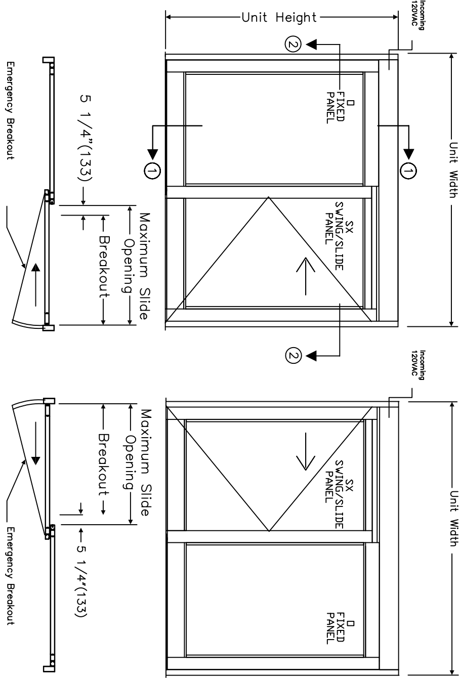
ELEVATION/PLAN TYPE O-SX and SX-O
