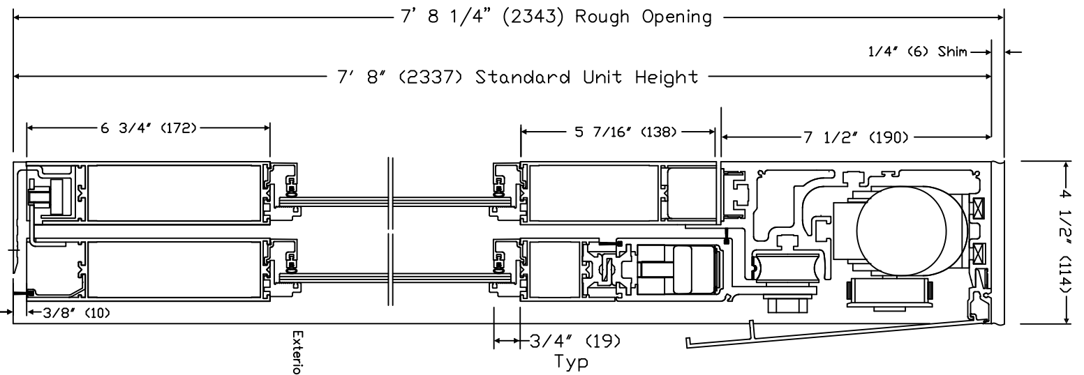
SECTION 1 TYPE O-SX, SX-O Door Shown in Open Position
