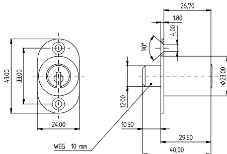
Type DRZ for furniture doors
