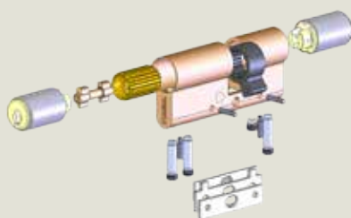
Increased protection against tearing and pulling with steel reinforcement and hardened tumbler pins and bolts
