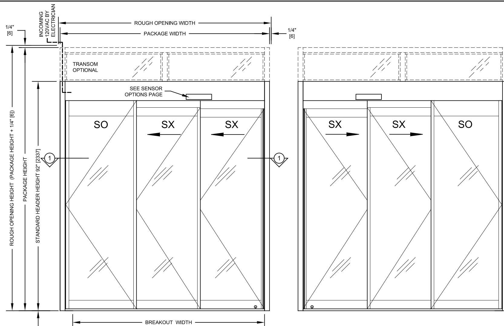
EXTERIOR ELEVATION TYPE: SO-SX-SX, SX-SX-SO
