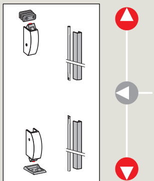
2/3-point locking
