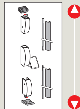
2-point locking
