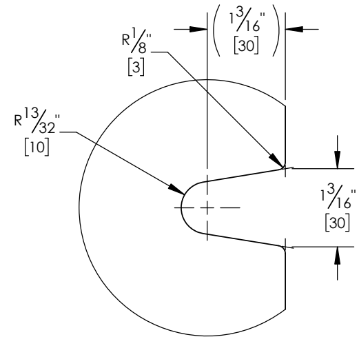
4X DETAIL A SCALE 1 : 2
