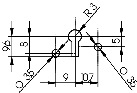
Fig. 1: Fastening hole pattern
