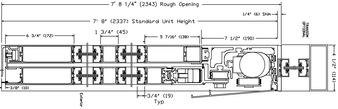
SECTION 1 TYPE O-SX, SX-O Door Shown in Open Position
