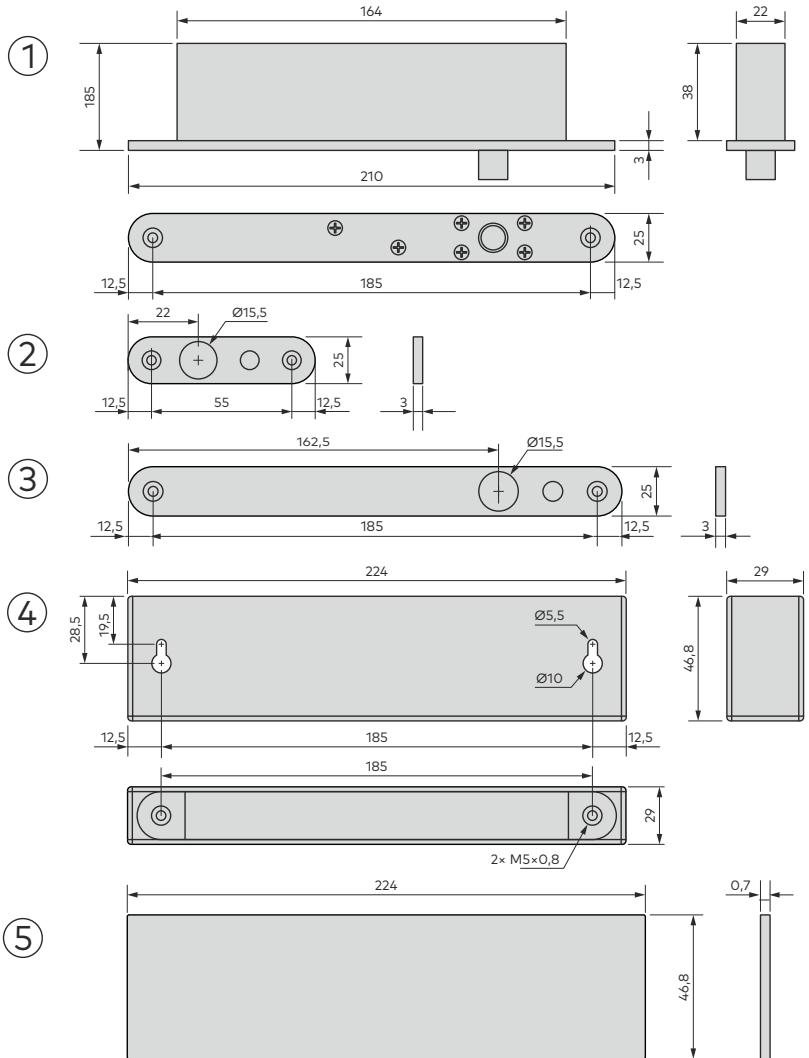
Fig. 2: Lock - dimensions
