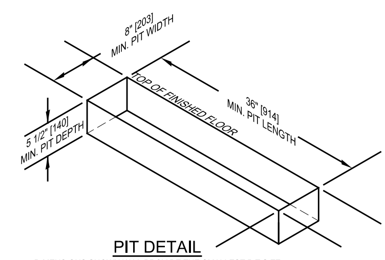
DIMENSIONS SHOWN WILL PROVIDE THE SMALLEST PIT SIZE
