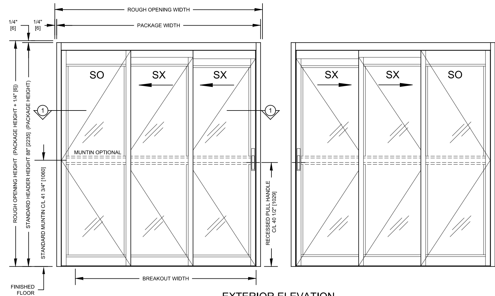
EXTERIOR ELEVATION TYPE: SO-SX-SX, SX-SX-SO
