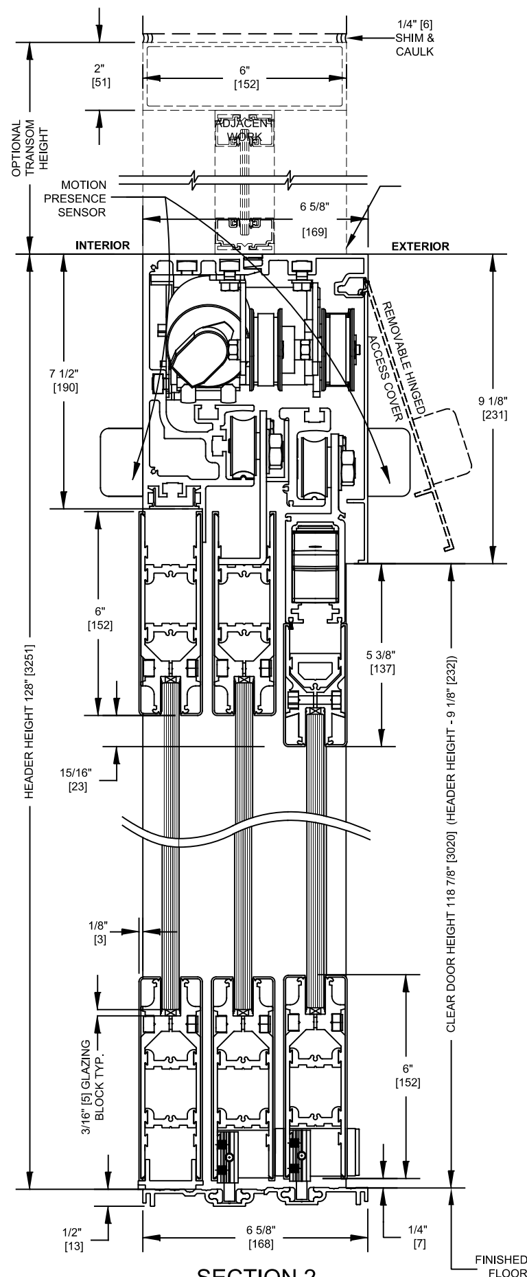
SECTION 2 TYPE: O-X2-SX1-SX1-X2-O
