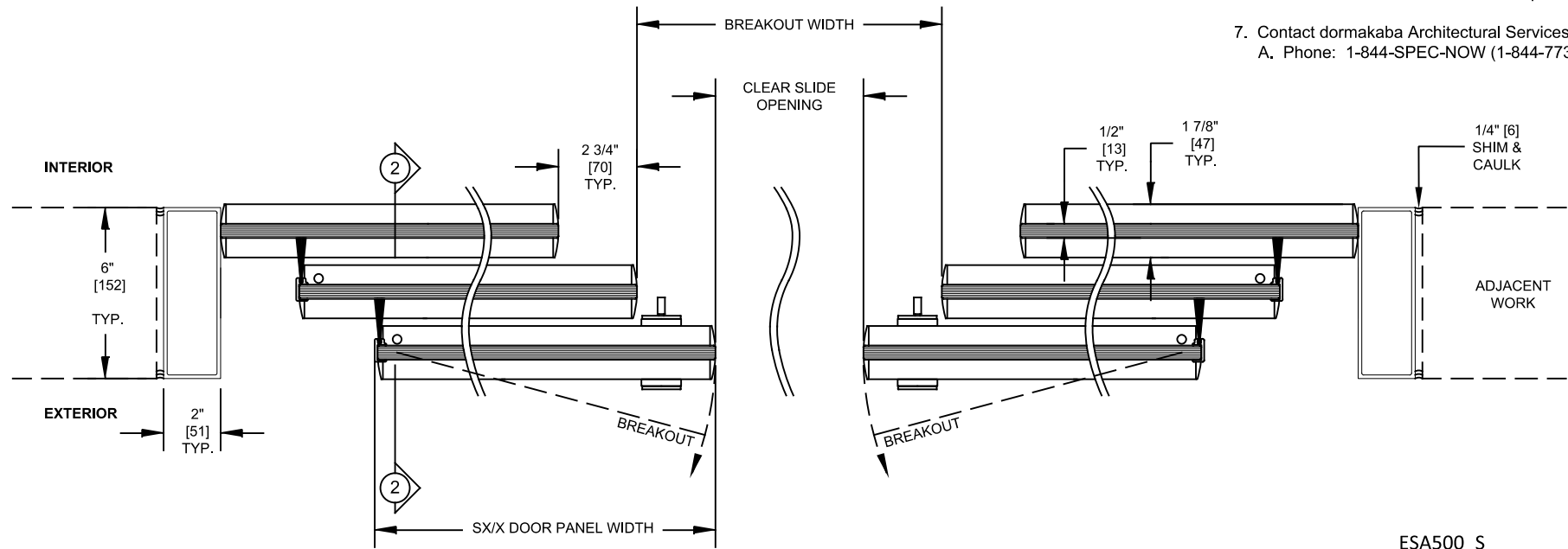
SECTION 1 TYPE: O-X2-SX1-SX1-X2-O
