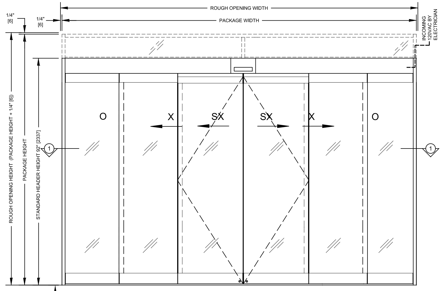
EXTERIOR ELEVATION TYPE: O-X2-SX1-SX1-X2-O
