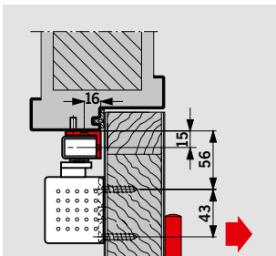
Angle bracket for G-N
