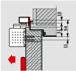
30 mm mounting backplate for G-N
