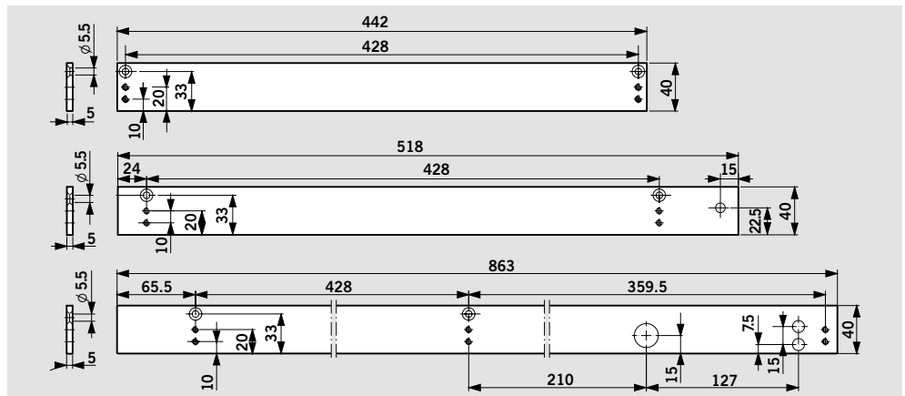
40 mm mounting backplate for G-N, EMF, EMR
