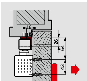
Angle bracket for G-EMF
