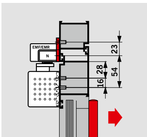
40 mm mounting backplate for G-N, EMF, EMR
