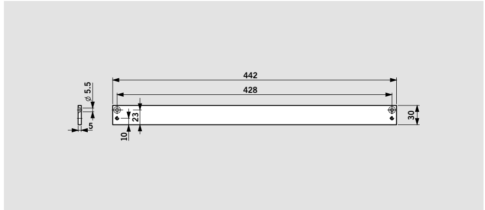
30 mm mounting backplate for G-N
