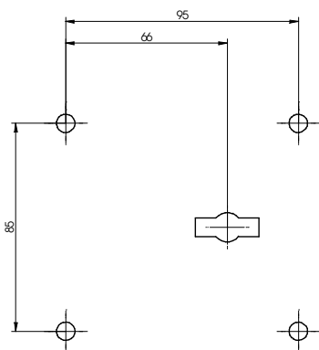
Fig. 3: Fastening hole pattern
