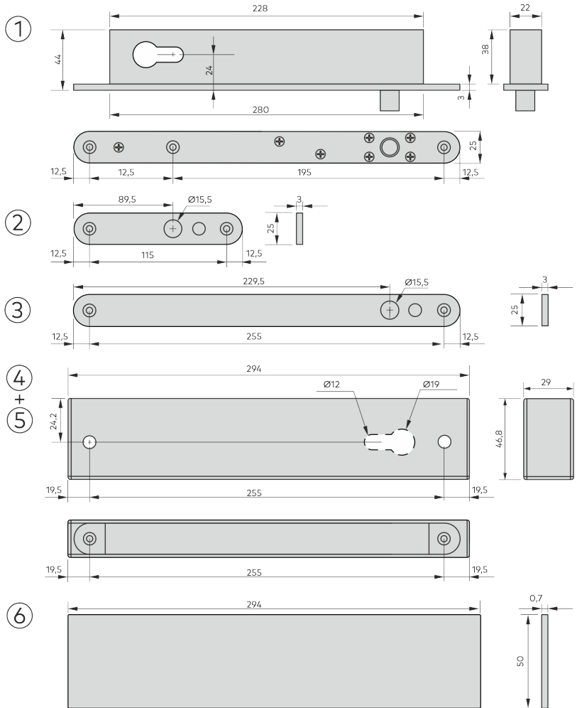
Fig. 2: Lock - dimensions
