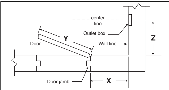
Figure 1. Locating the Door Holder
