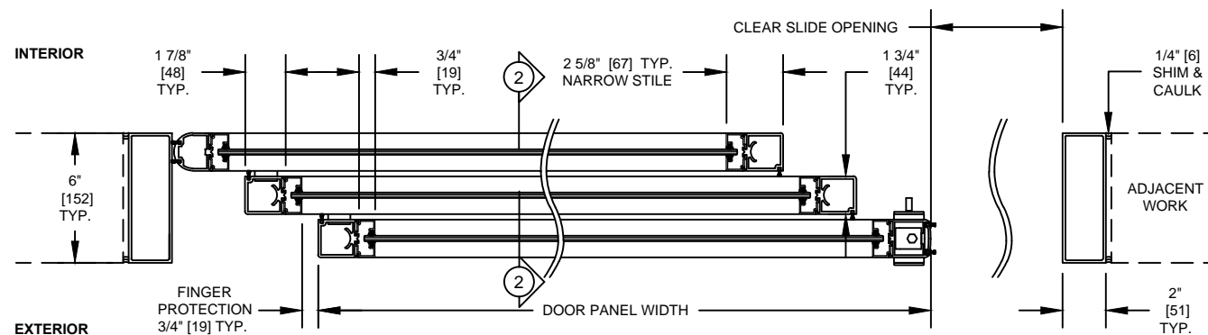
SECTION 1 TYPE: O-X-X SHOWN, X-X-O OPPOSITE DOOR SHOWN IN OPEN POSITION WITHOUT THRESHOLD
