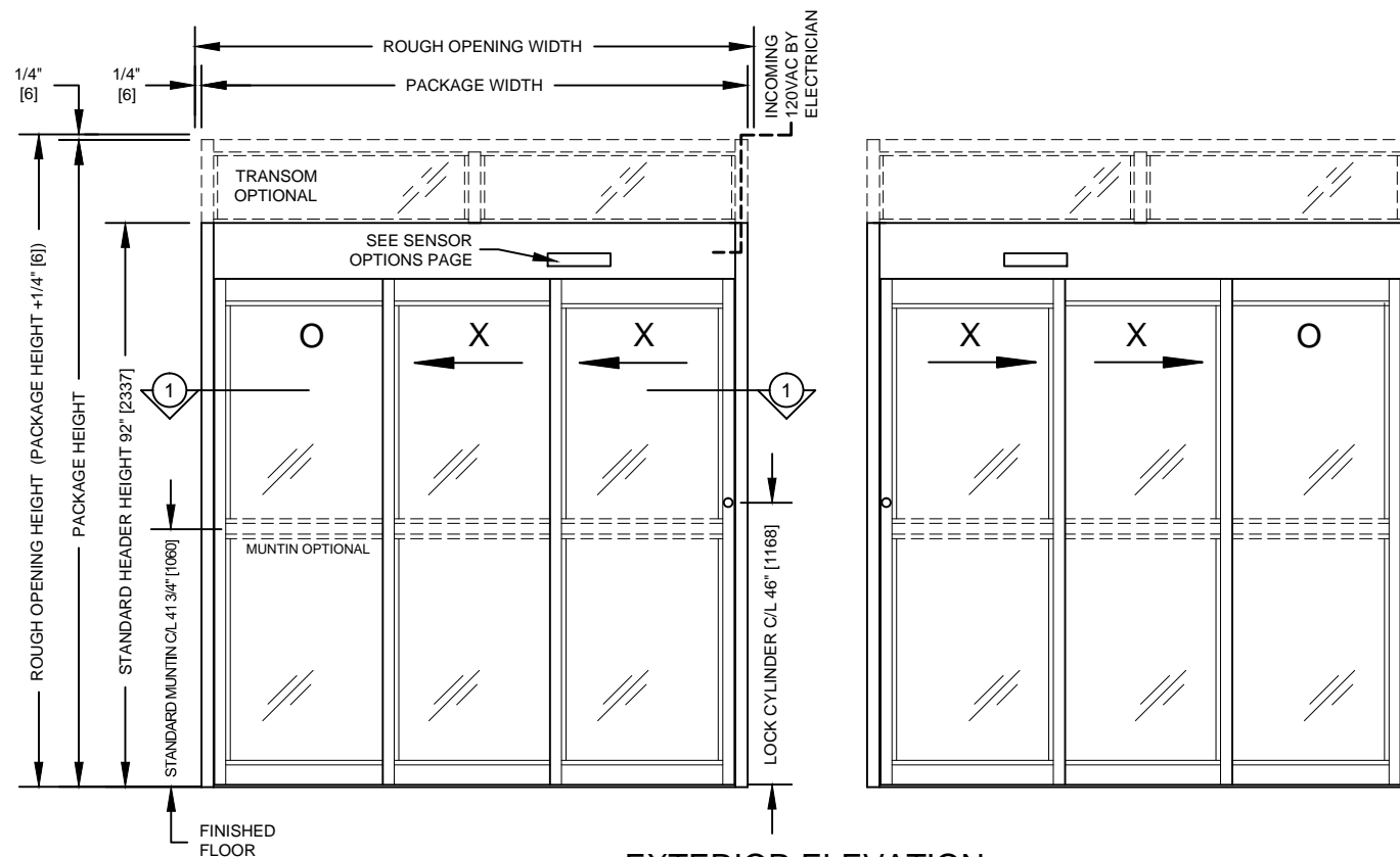
EXTERIOR ELEVATION TYPE: O-X-X, X-X-O
