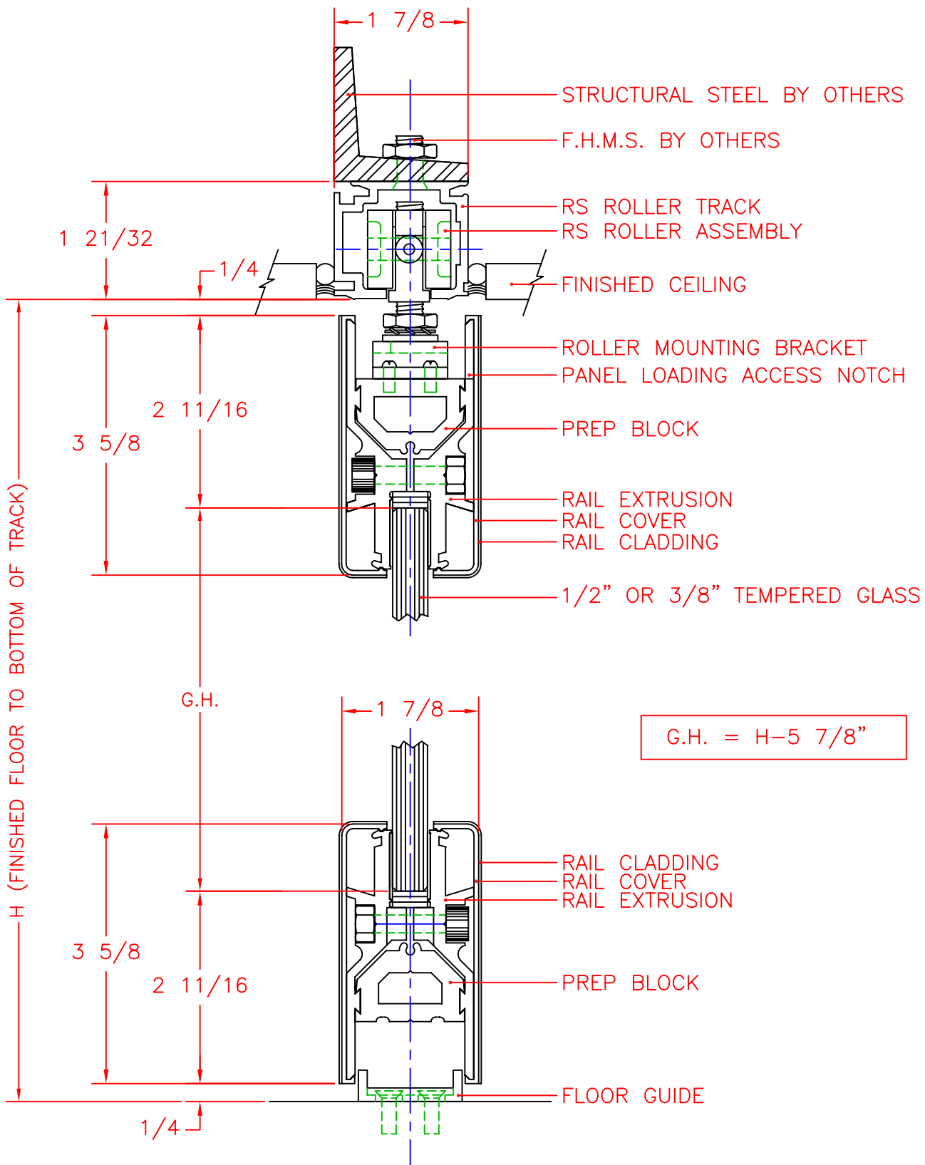
RS-DRS SECTION THRU SLIDING PANEL
