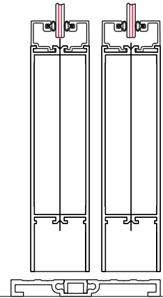
(Optional) Recessed Threshold 1/2" x 4-1/2"
