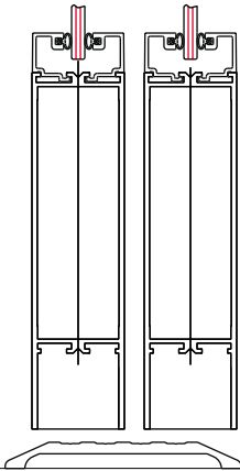
Standard Threshold 1/2" x 4-1/2"
