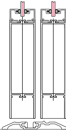
Standard "SO" Track 1/2" x 4-1/2"
