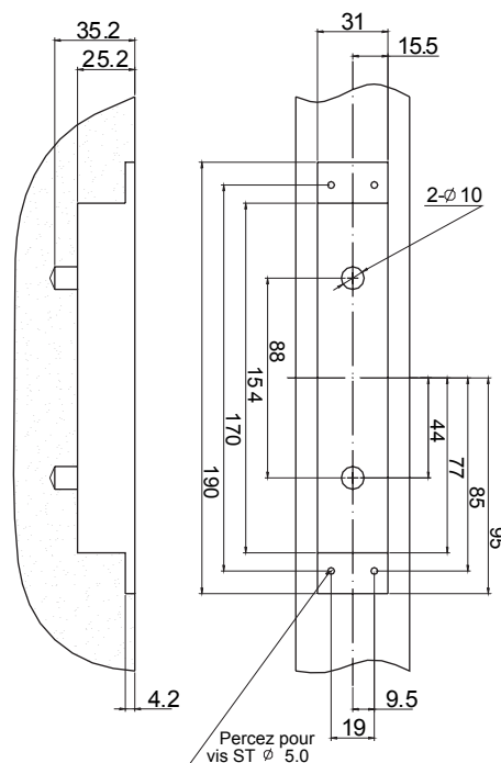
Typical installation for wooden door (GB)
