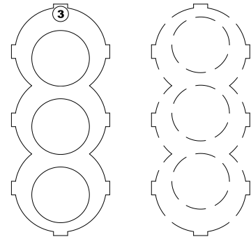
Bushing #3
