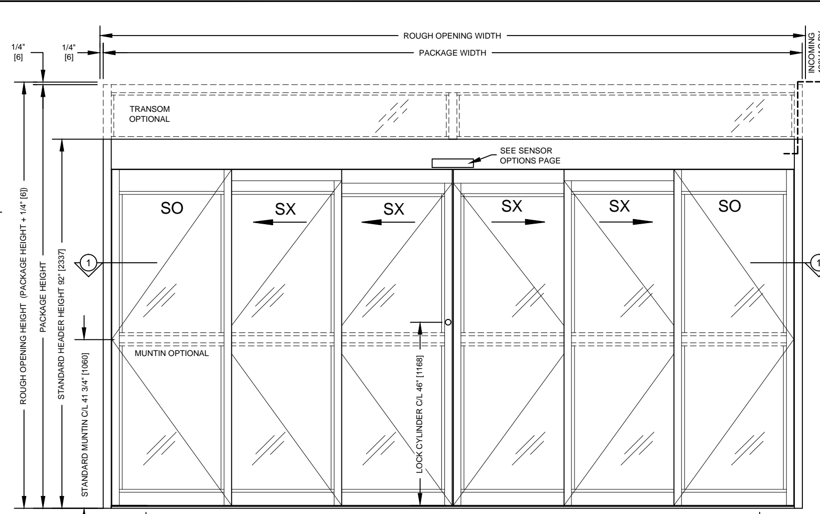
EXTERIOR ELEVATION TYPE: SO-SX-SX-SX-SO
