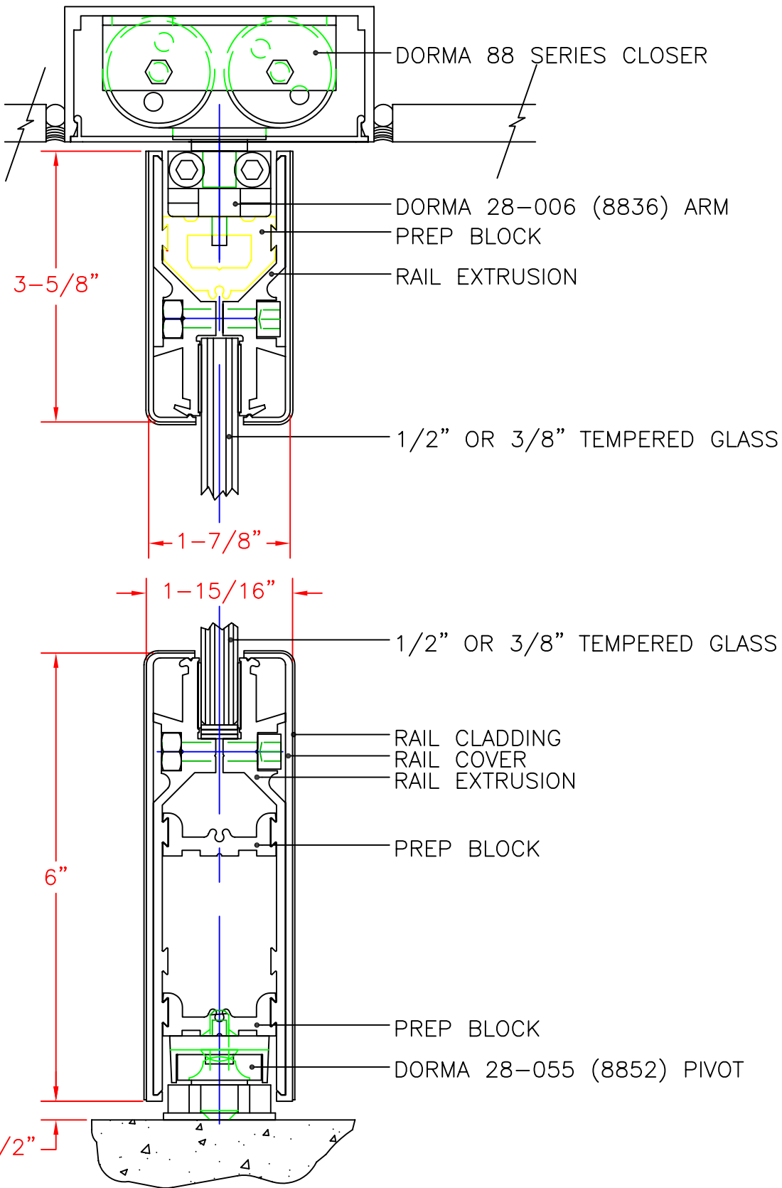
SECTION THRU DOOR AND RTS CLOSER
