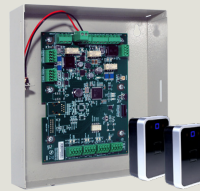
RAC5 Lite (offline only) with RAC5 RFID readers
