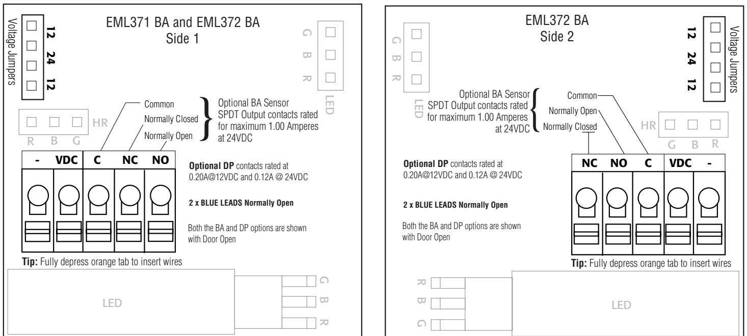
Figure 2. Wiring : For BA or BA DP Combination Models
