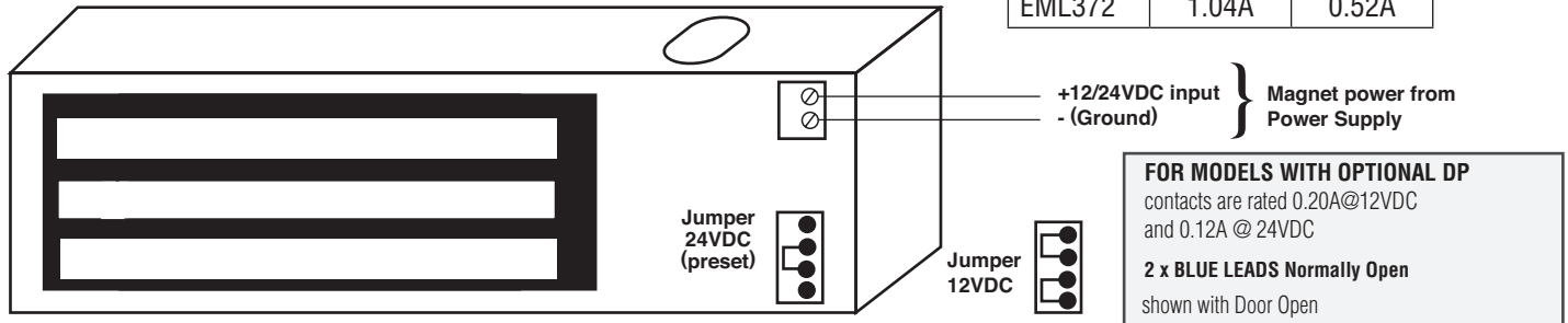
Figure 1. Wiring : For Unmonitored or DP Sensor Models
