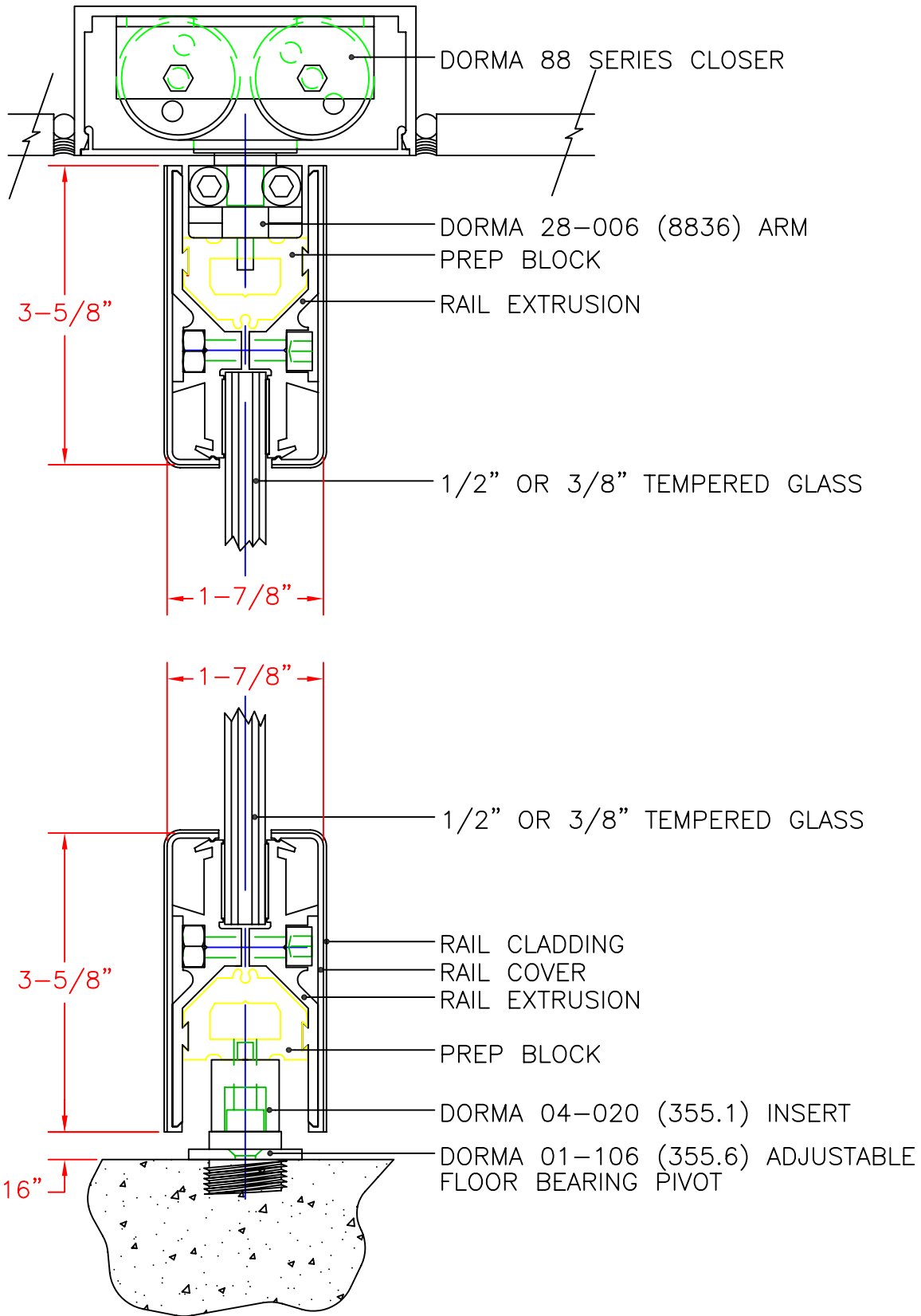
SECTION THRU DOOR AND RTS CLOSER
