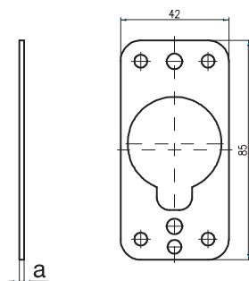
Support plate
